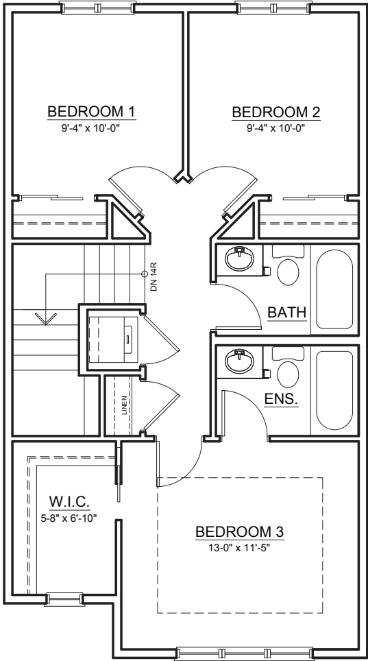
UPPER FLOOR OPTION 2
