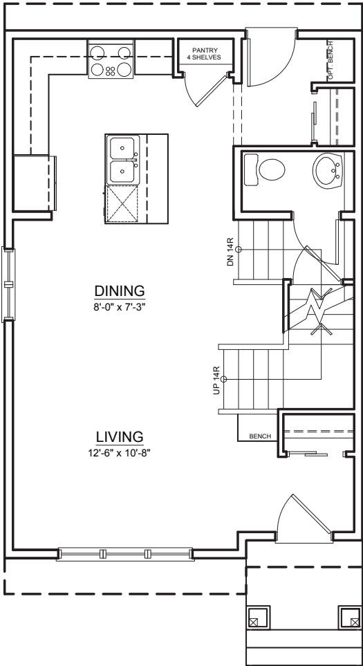
MAIN FLOOR ± 584 SQ. FT.
