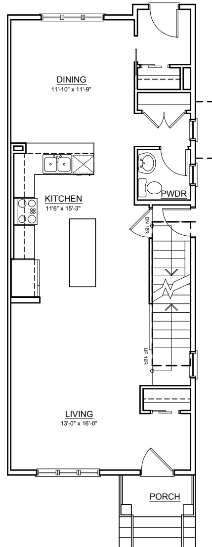
MAIN FLOOR ±798 SQ. FT.
