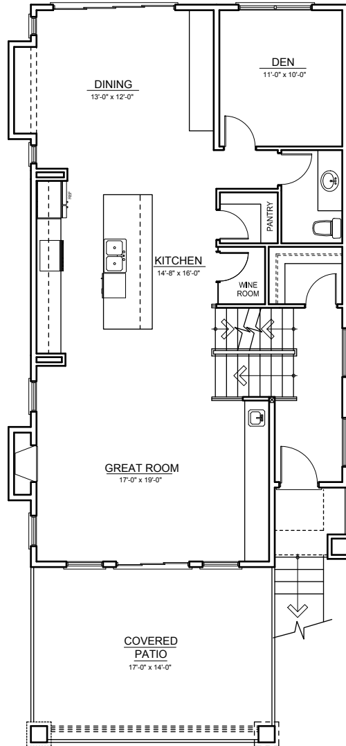
MAIN FLOOR ±1,183 SQ. FT.
