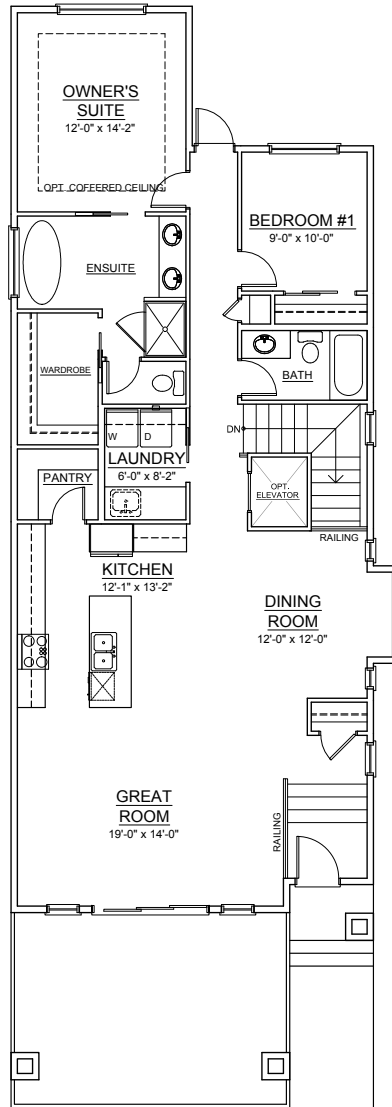
MAIN FLOOR ± 1,621 SQ. FT.
