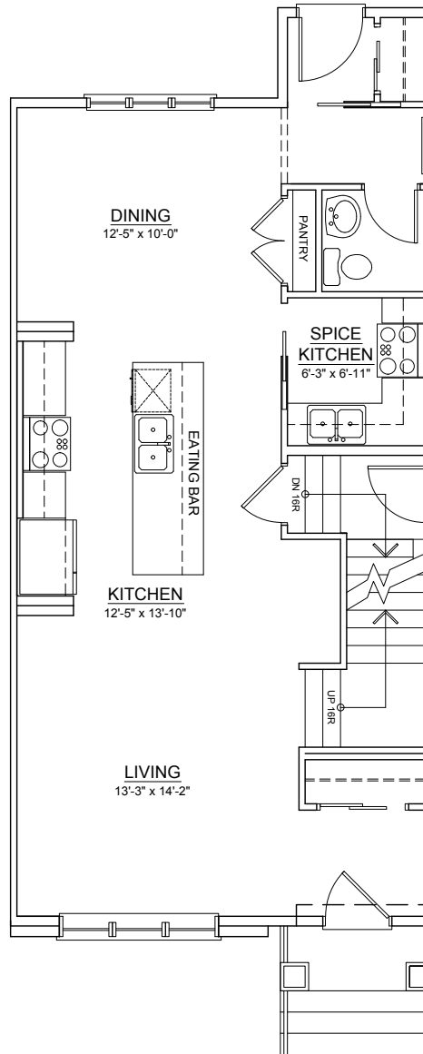
MAIN FLOOR OPTION 3 ±814 SQ. FT.
