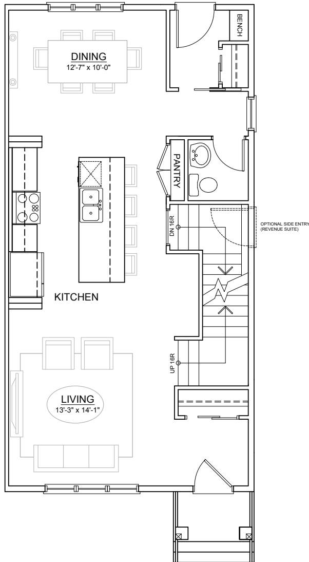
MAIN FLOOR OPTION I ±778 SQ. FT.
