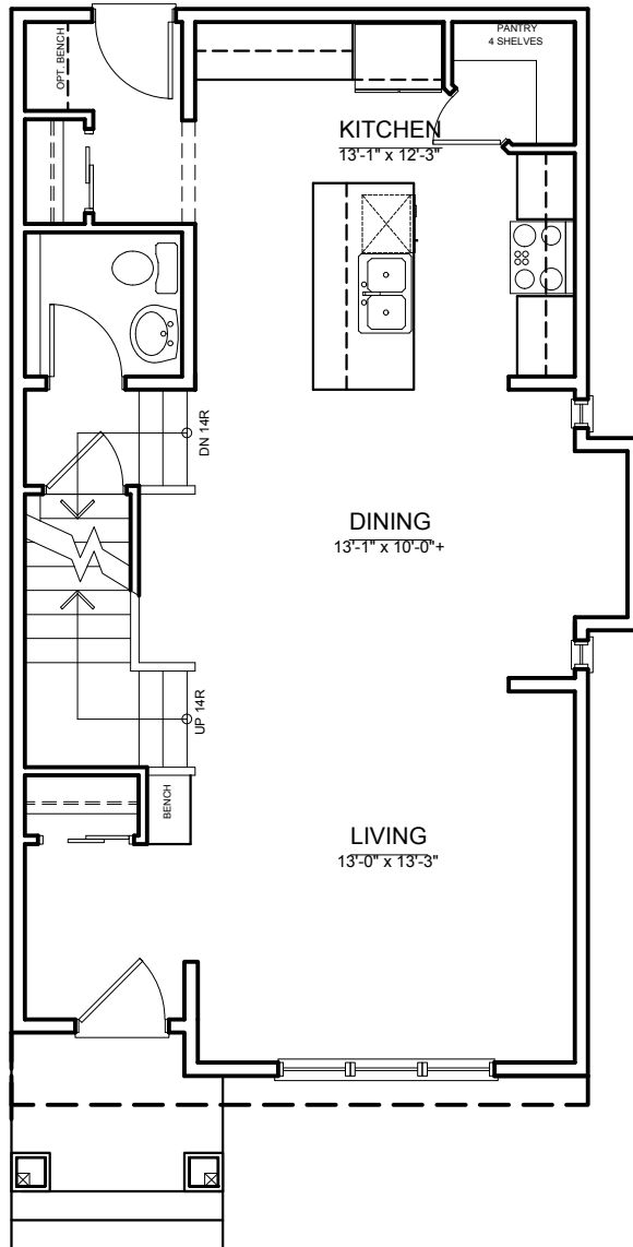
MAIN FLOOR ±731 SQ. FT.
