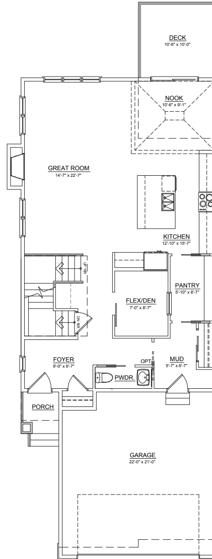
MAIN FLOOR 1091 SQ. FT.
