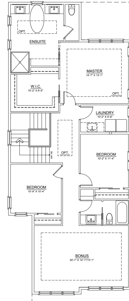
UPPER FLOOR 1420 SQ. FT.
