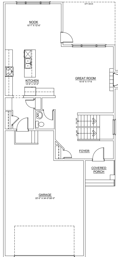
MAIN FLOOR 1006 SQ. FT.
