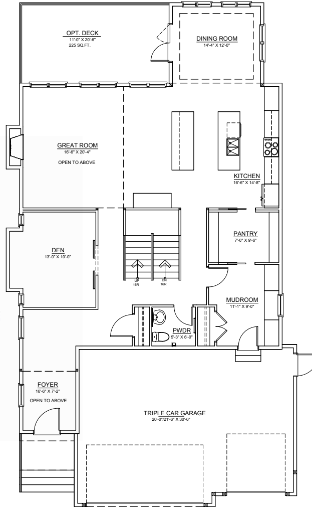
MAIN FLOOR 1576 SQ. FT.
