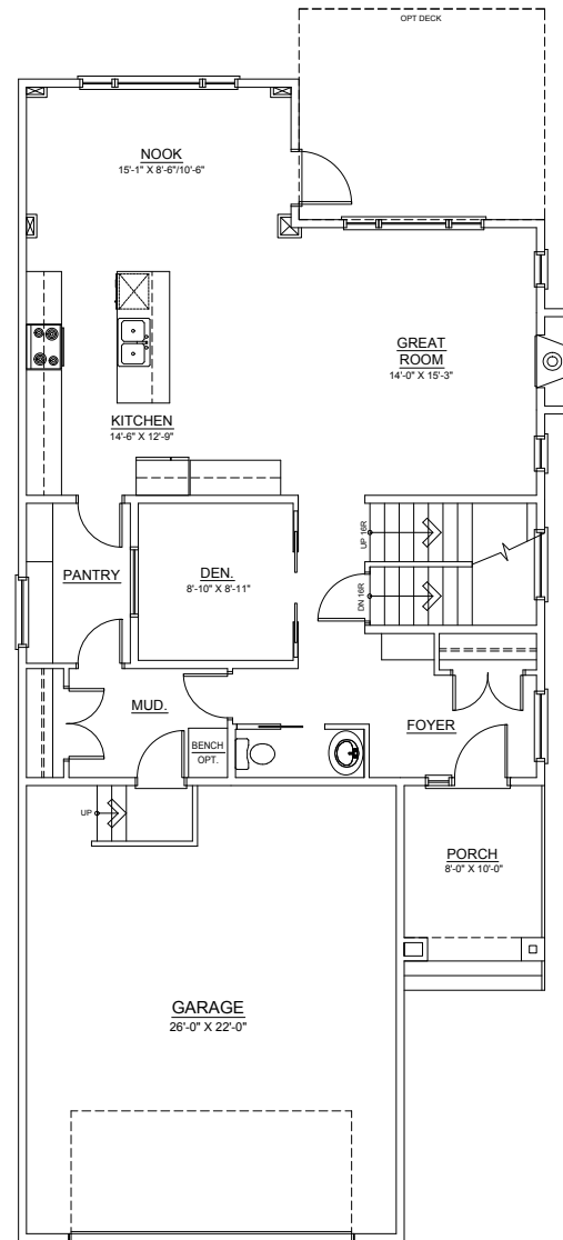
MAIN FLOOR 1098 SQ. FT.
