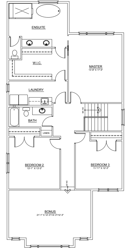
UPPER FLOOR 1575 SQ. FT.
