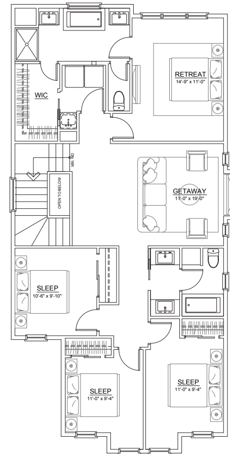
UPPER FLOOR 1276 SQ. FT.
