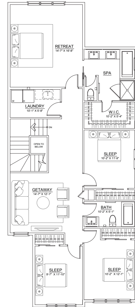
UPPER FLOOR 1411 SQ. FT.
