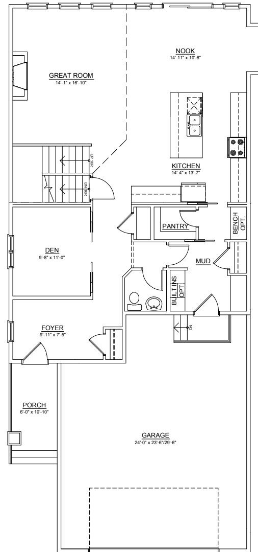
MAIN FLOOR 1284 SQ. FT.
