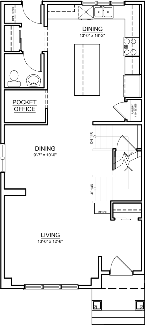
MAIN FLOOR OPTION 2
