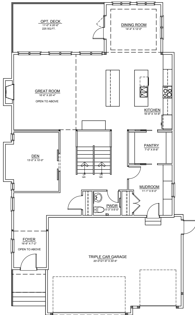
MAIN FLOOR 1576 SQ. FT.
