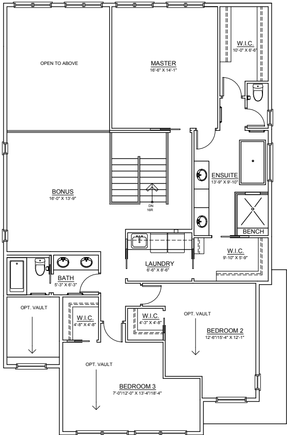
UPPER FLOOR 1665 SQ. FT.
