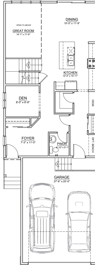
MAIN FLOOR ±985 SQ.FT.
