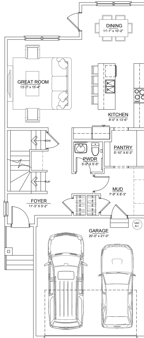
MAIN FLOOR ±868 SQ.FT.
