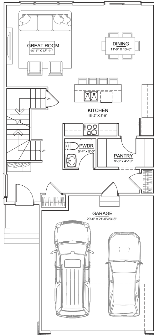
MAIN FLOOR ±880 SQ.FT.
